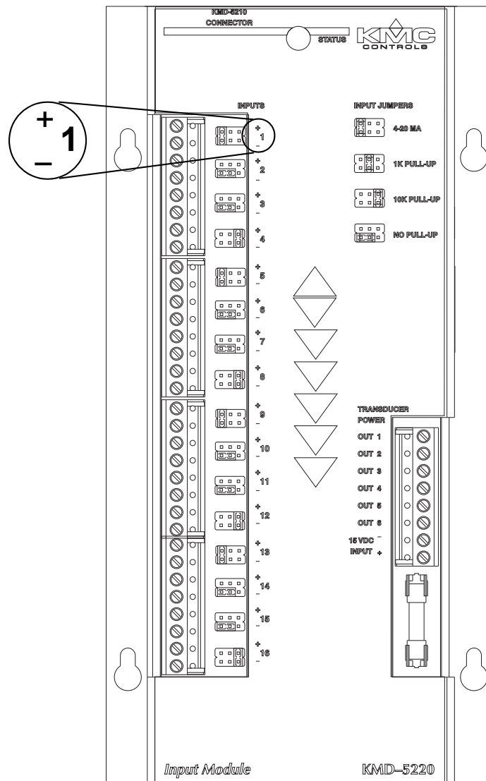
Illustration 1 KMD-5220 polarity markings
